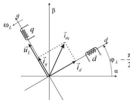
Fig. 1 Synchronization of the d - q frame to the line voltage [10].
