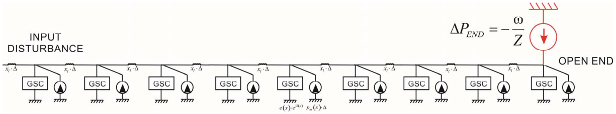
Fig. 6. A total of 64 inverters (GCS) are connected in series. The input disturbance is applied to the leftmost node in the form of a 500 ms wide power pulse. The rightmost node could be left open, or, supplied by the impedance-matching power source that quenches the reflection of the electronic power waves.
