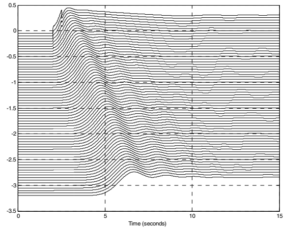
Fig. 8. In addition to settings of Fig. 7, the impedance-quenching compensation is applied at the right end of the string, providing the power pulse that rests in proportion with the phase-shift deviation.
